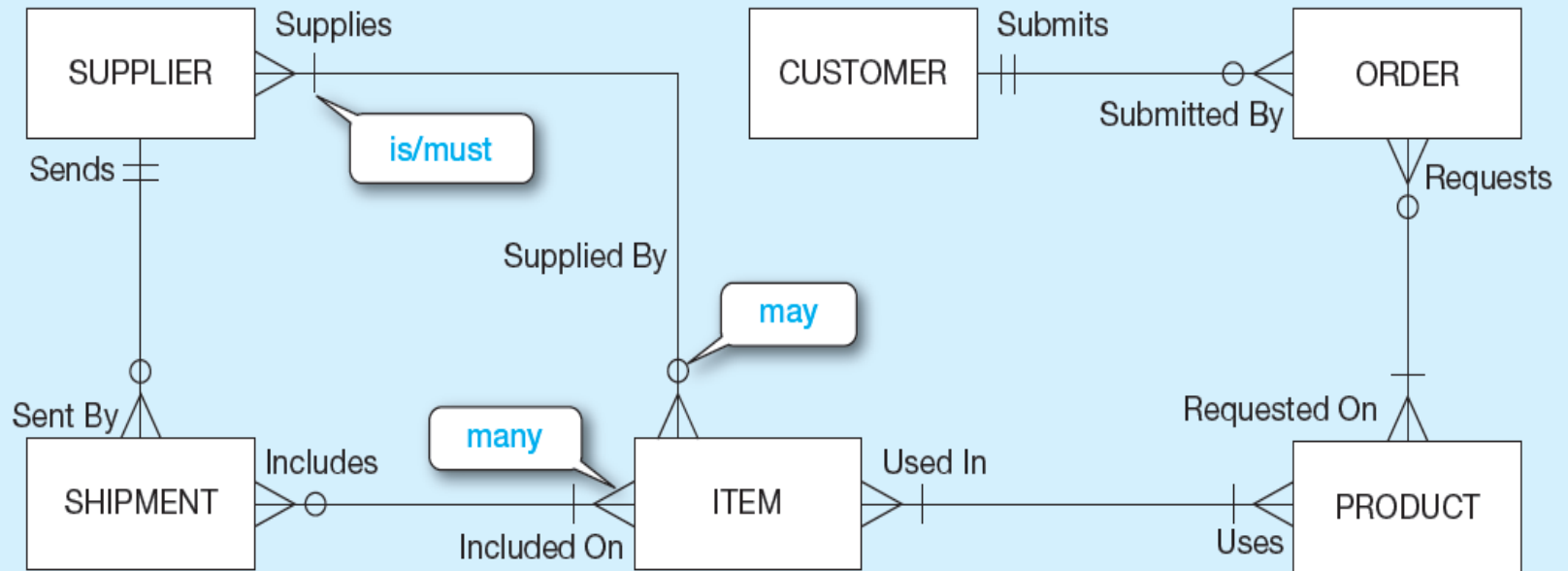
Figure 2-1 Sample E-R Diagram
