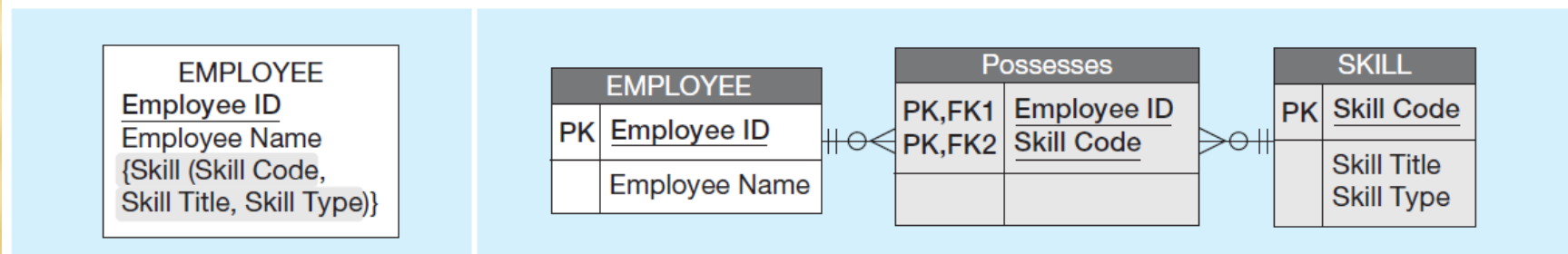
(b) Composite, multivalued attribute versus relationship
