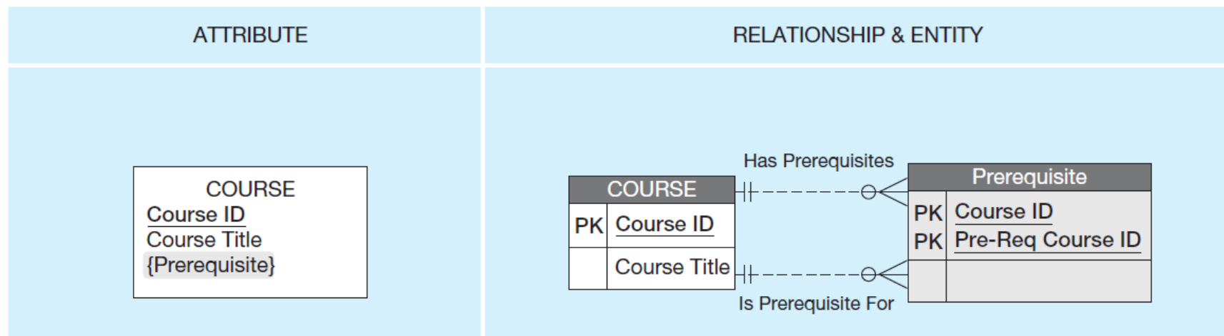
(b) Composite, multivalued attribute versus relationship
